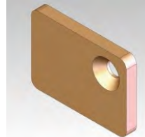
6 Shooter Right Side Guide, Brass 3/16 X 1-1/4 X 1-3/4.
