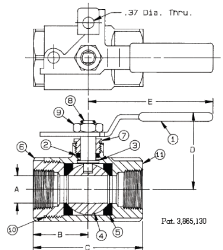
BRONZE PAD LOCKING BALL VALVE
