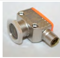
Diffuse Photo Eye 24 Volts DC 8" (200MM) With Background Suppres- sion Right Angle 18MM Dia. IFM Effector (Uses M12 4 Pin Cord Not Included) KVAL P/N: OGH283
