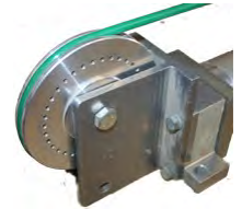
Cylinder, Modified Cable Greenco Cable-Trol, CD 3226, Modified End Pulley and Housing to accommodate Photo Emitter and Receiver
