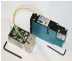
Single Valve and Adapter Plate ASSY, 120V, 4 Way Single Acting (SMC MFG P/N NVS4114 Replacement) Substitute for: SMCNVS401 KVAL P/N: MAC-92-SINGLE-120V-NVS
