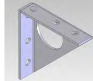
SAFETY CAGES, CORNER BRACKET, CRS 11GA (.119), ZINC COATED.
